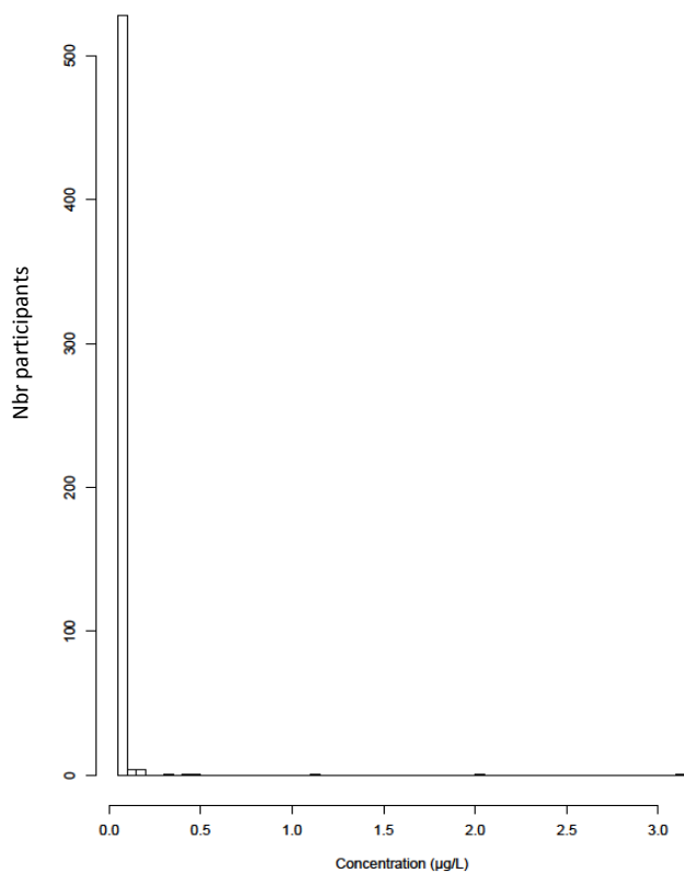
4-F-3-PBA
