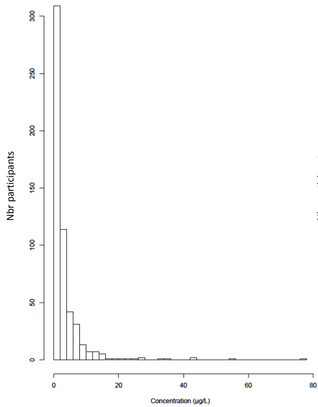
DEDTP
