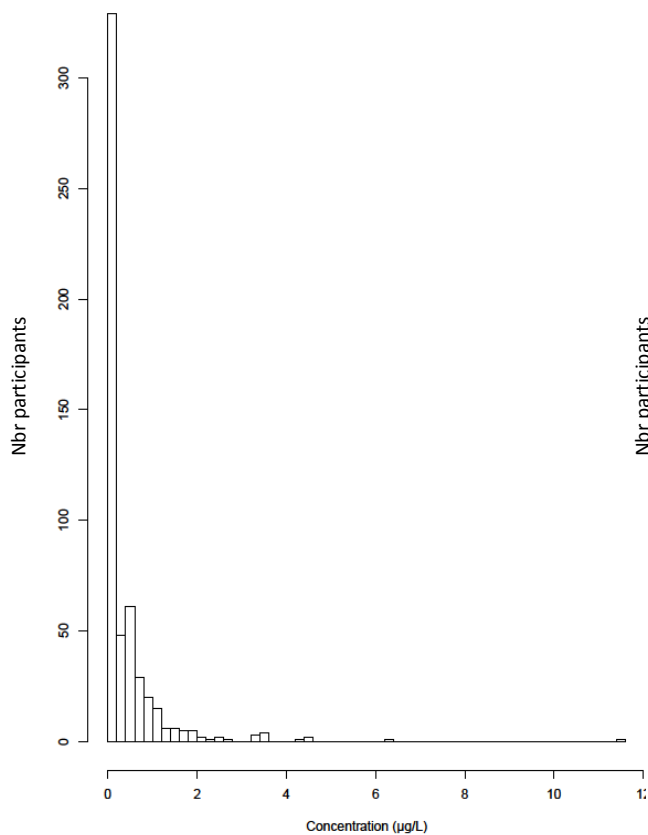
4-F-3-PBA
